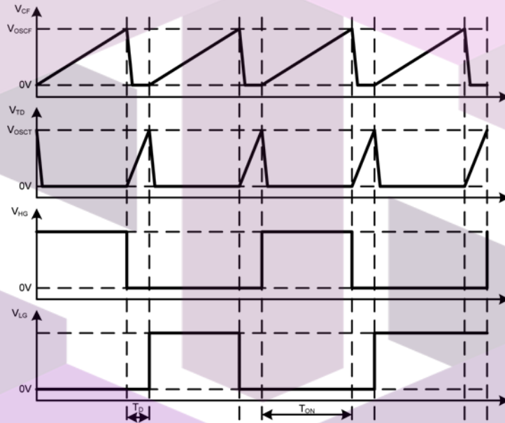
Figure 5 Oscillator waveforms
